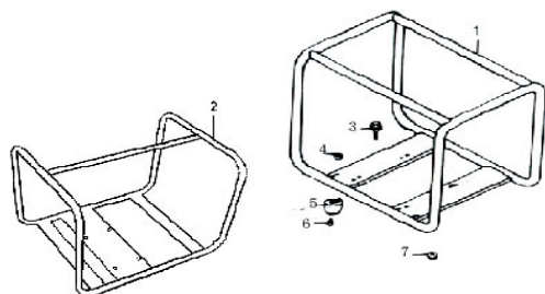
2寸水泵 ( 2" PUMP )
