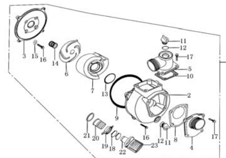
3寸水泵 ( 3" PUMP )
