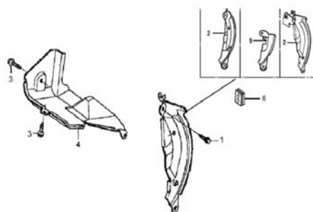
导风部件(DIVERSION ASSY.)
