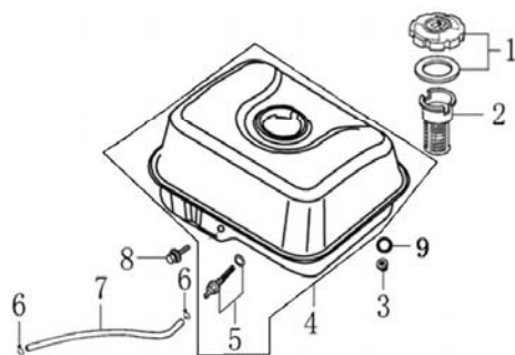
3寸水泵 ( 3" PUMP )
