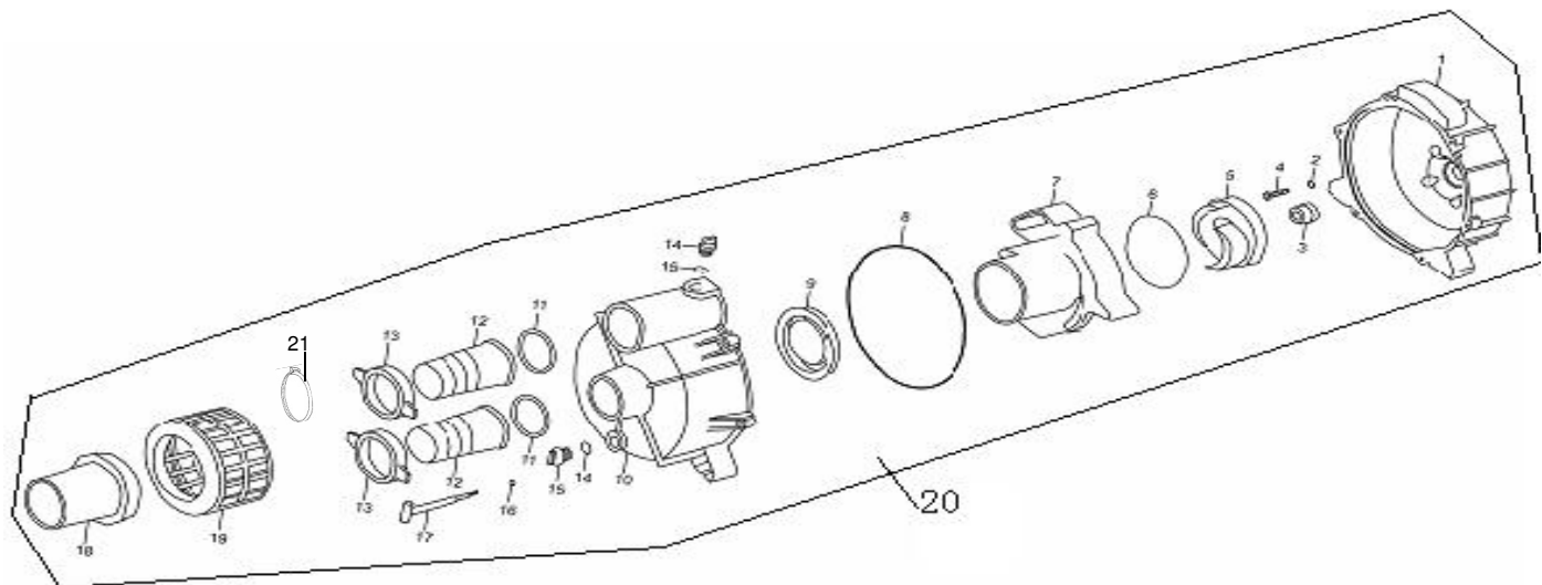
排污泵 ( TRASH PUMP )
