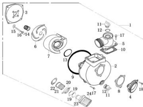
3寸水泵 ( 3" PUMP )
