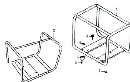
3寸水泵 ( 3" PUMP )
