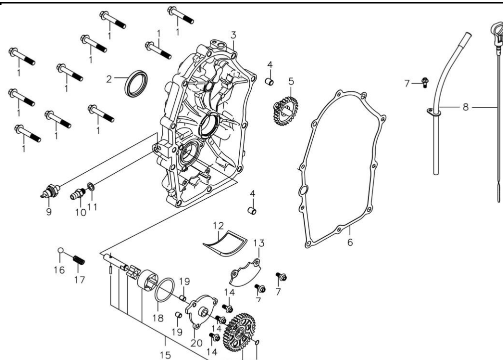
曲轴箱盖 (CRANKCASE COVER)
