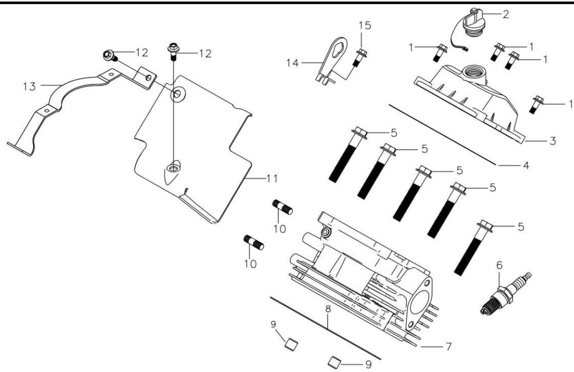
气缸头II总成 (CYLINDER HEAD ASSY)
