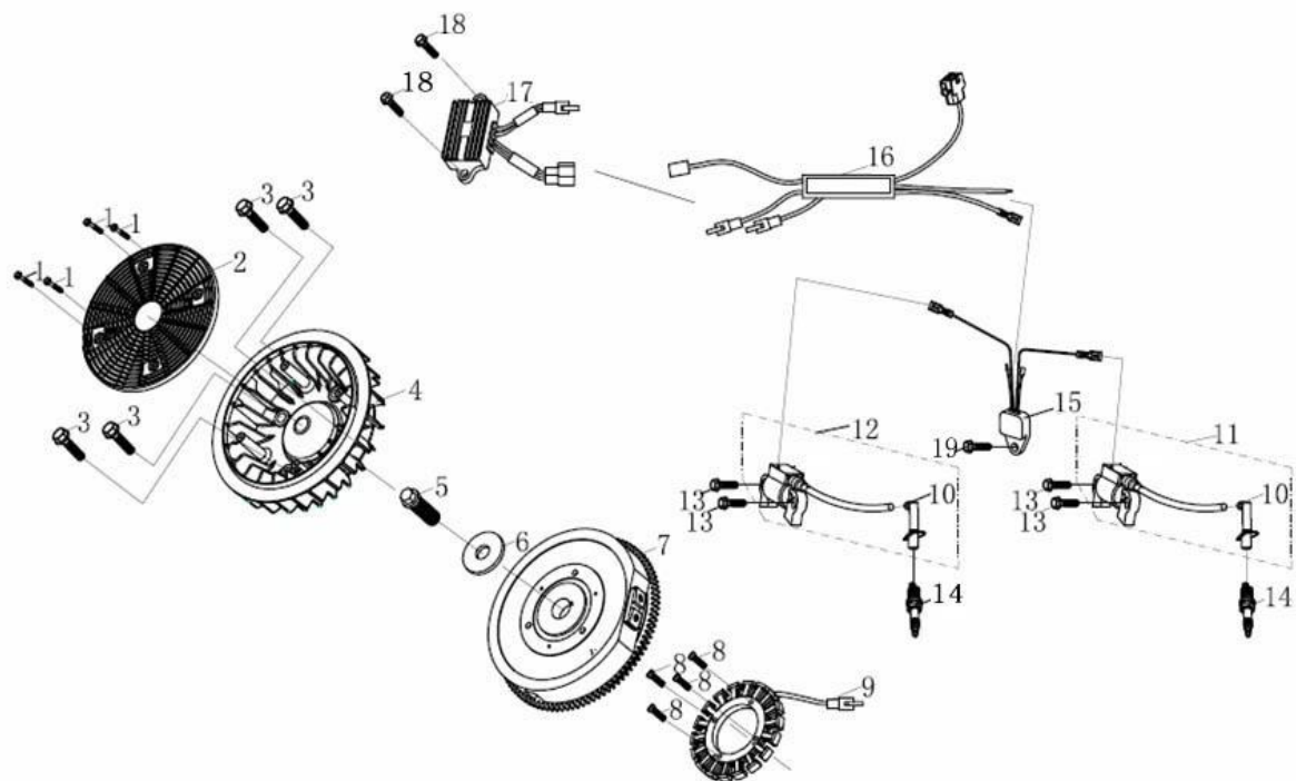
飞轮/点火器线圈 (Flywheel/Coil Assy.)
