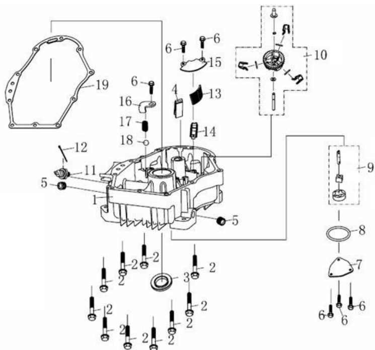
箱盖 (Crankcase Cover)
