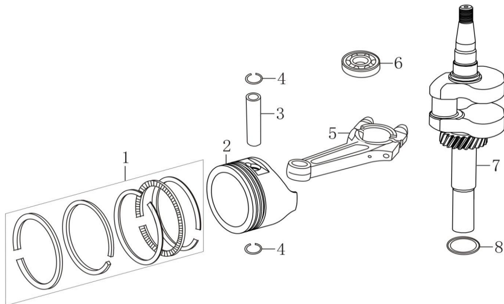
曲轴/活塞 (CRANKSHAFT/PISTON)
