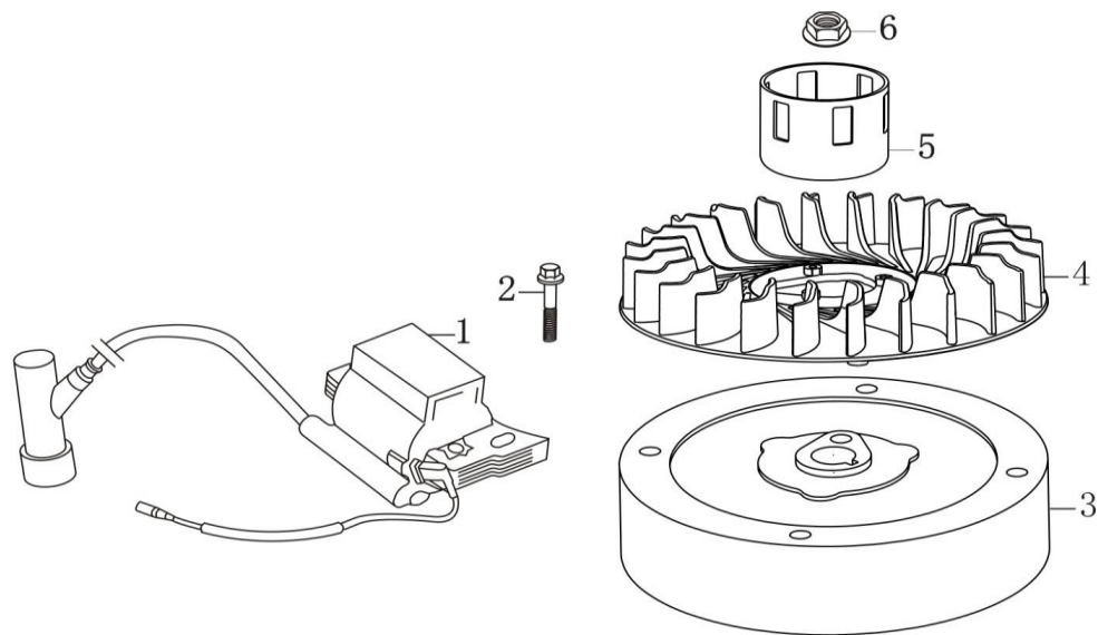
飞轮 点火器 (FLYWHEEL/IGNITION COMP)
