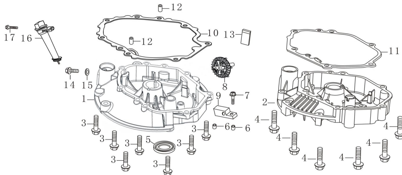
曲轴箱盖 (CRANKCASE COVER)
