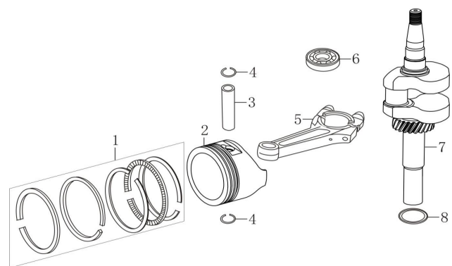
曲轴/活塞 (Crankshaft/piston)
