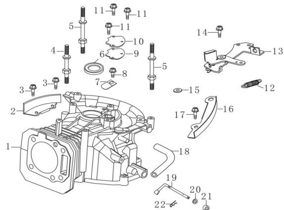
曲轴箱 (Crankcase)
