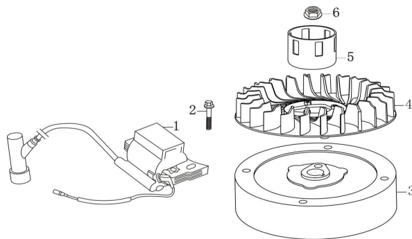
飞轮 点火器 (Flywheel/Ignition Comp)
