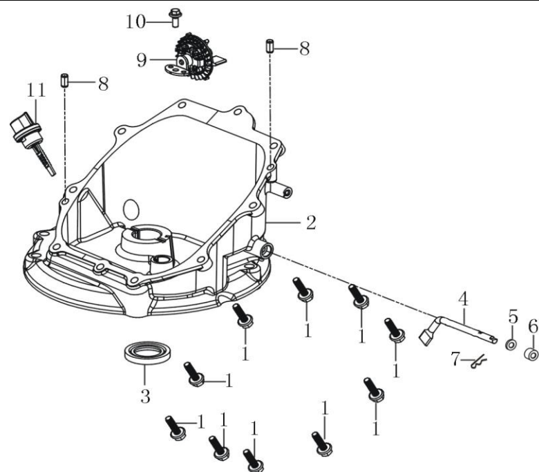
曲轴箱盖 (CRANKCASE COVER)
